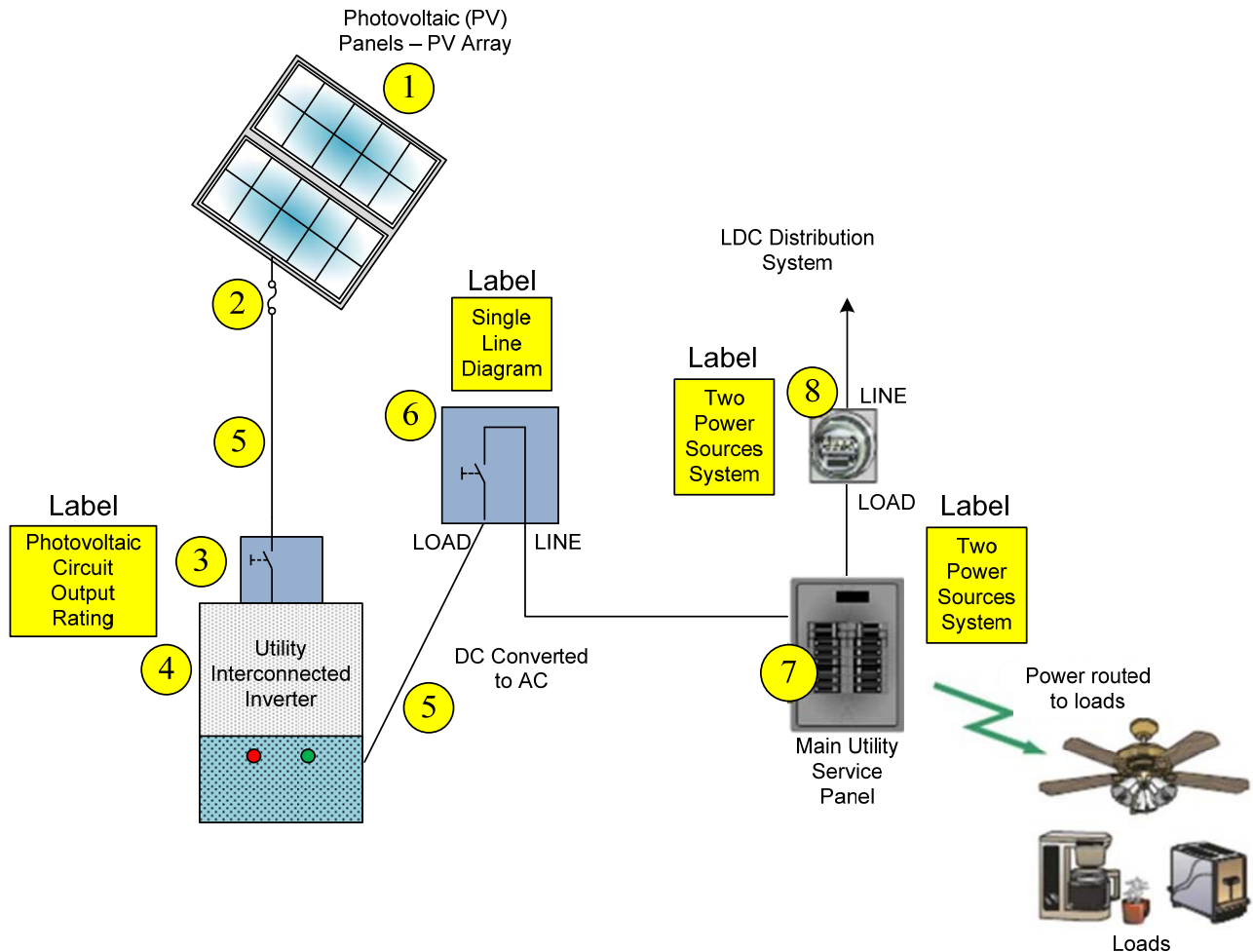
Diagram C: Net metering connection - Micro-embedded Load Displacement project
